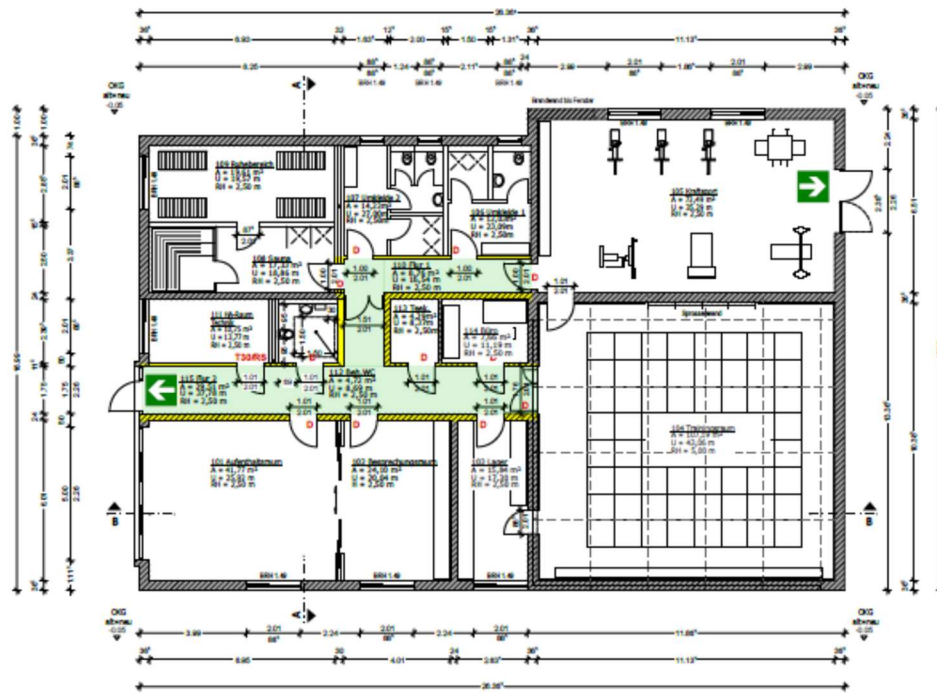
GRUNDRISS TKZ
